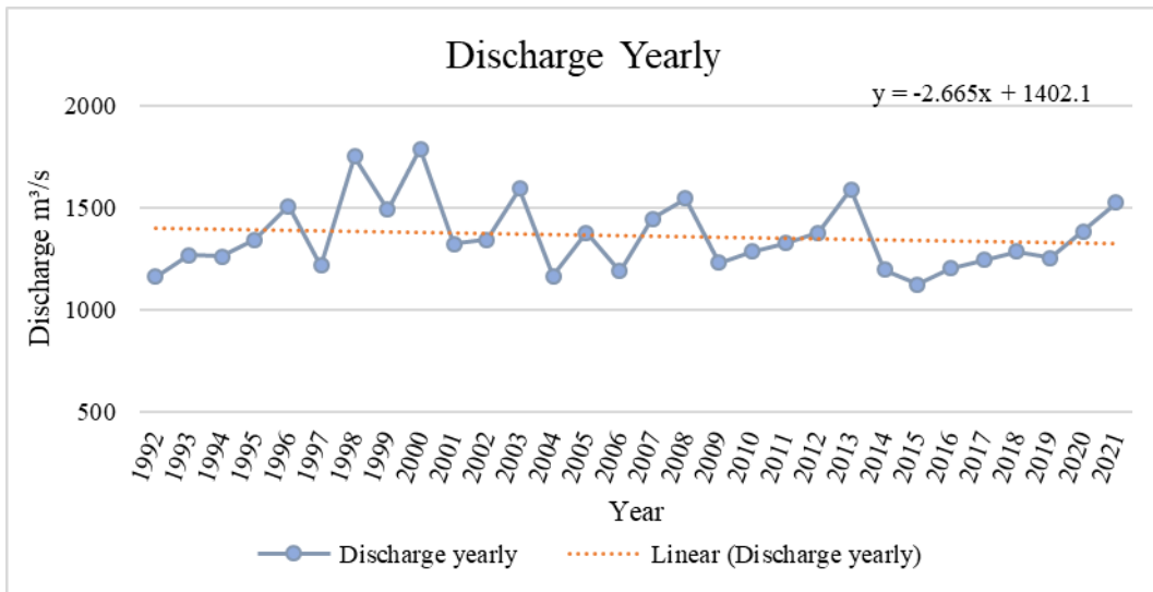
Figure 20: Annual Discharge
