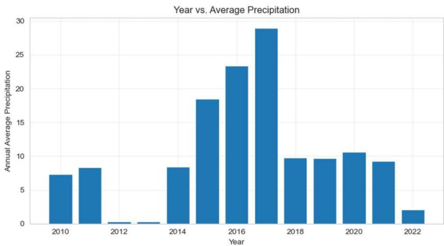
Figure 3: Year vs Average Precipitation
