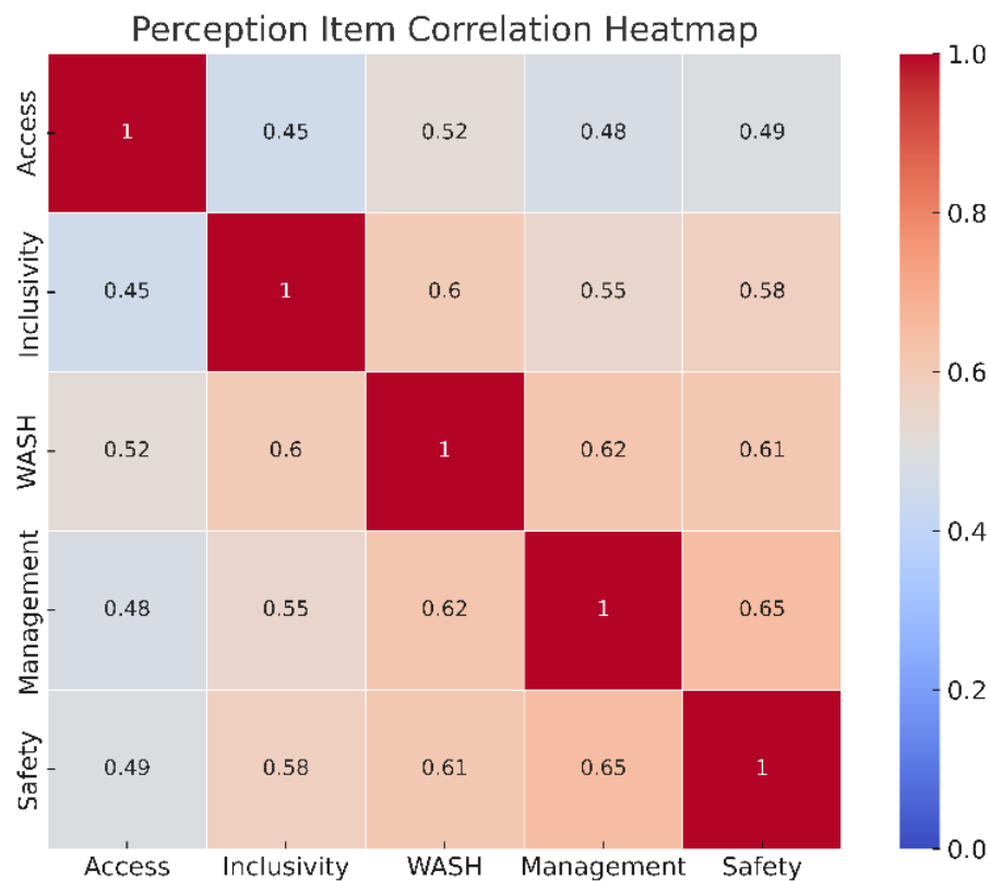
Figure 2: Heatmap of perception item correlations
