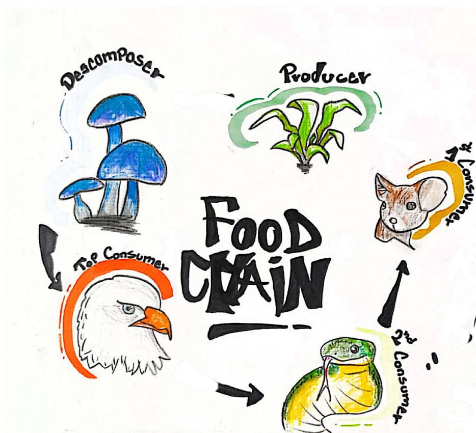
Image 1: Food chain and trophic levels.
