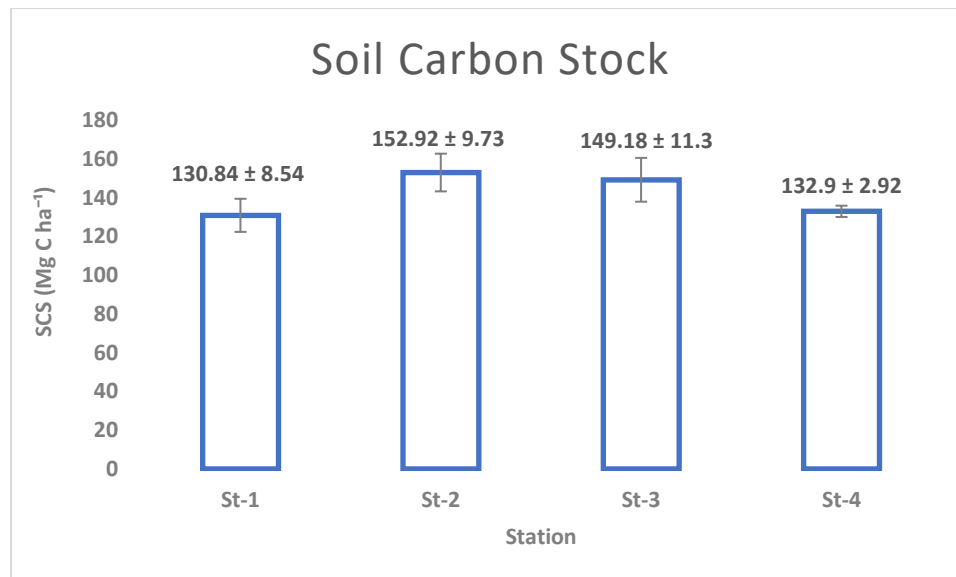
Figure 2: Mean soil carbon stock ( \text{Mg C ha}^{-1} ) across four sampling stations.
