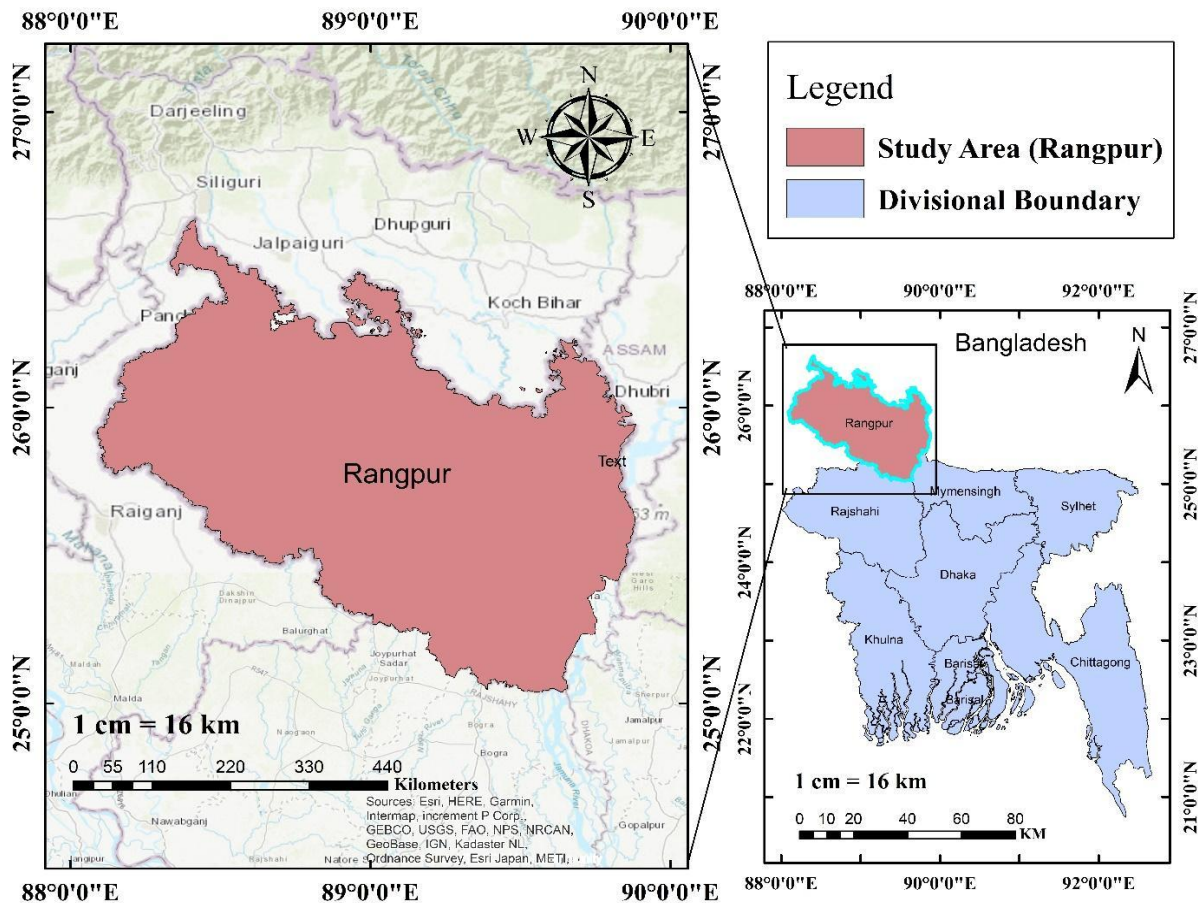
Figure 1: Location of the Study Area (Rangpur Division)
